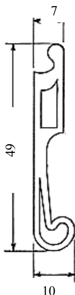
Joint de Porte Ref. JG-4950
